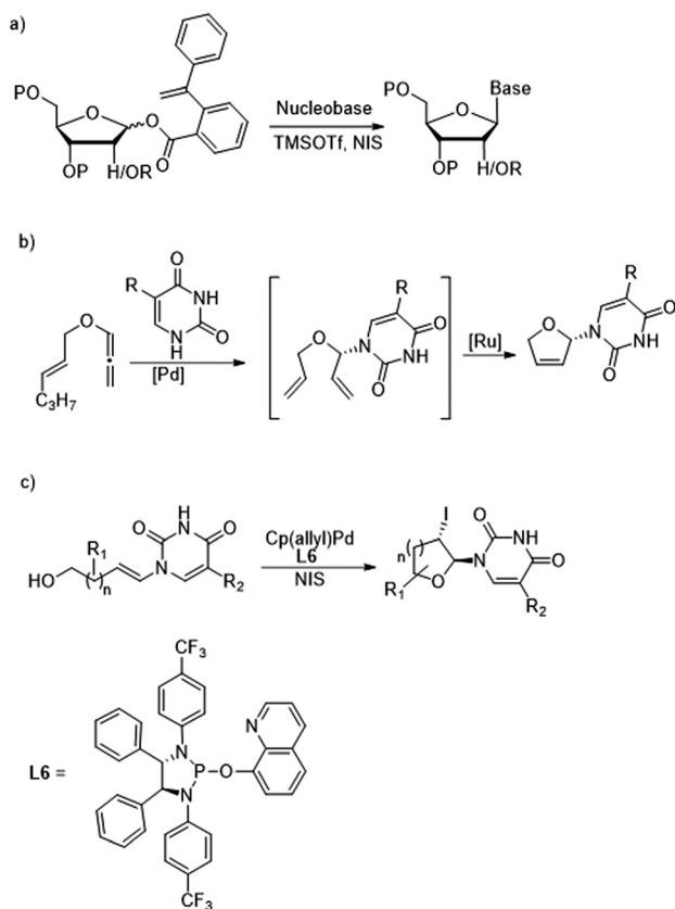
Fig. 4 Recent alternative glycosylation reactions: (a) broad scope method based on a stable O -glycosyl donor; 93 (b) sequential metal catalysis method using unprotected nucleobases; 46 (c) asymmetric Pd-catalyzed iodoetherification method. 38
