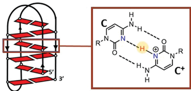
Fig. 16 Schematic of i-motif and illustration of a hemi-protonated cytosine-cytosine base pair.
