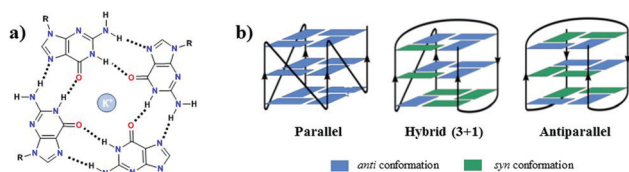
Fig. 12 (a) G-tetrad with a central potassium ion; (b) different G-quadruplex topologies.
