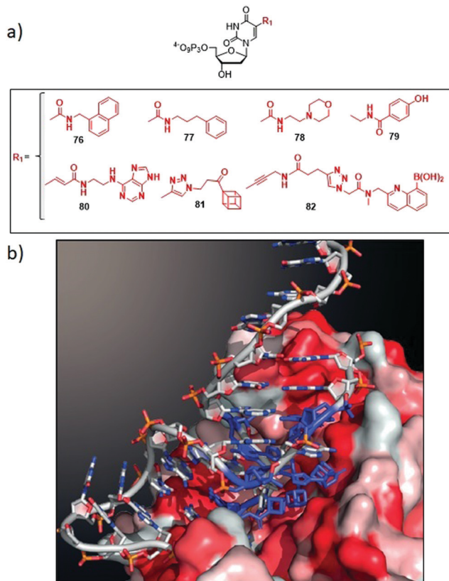
Fig. 23 (a) Chemical structures of base-modified nucleoside triphosphates used in aptamer selections; (b) X-ray structure of a cubane-modified aptamer in complex with the protein PvLDH (PDB ID code: 6TXR; courtesy from Dr Pascal Röthlisberger).
