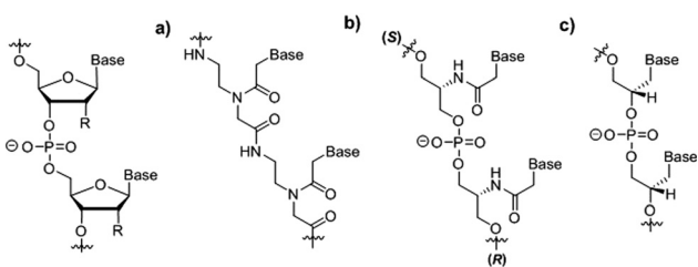
Fig. 6 Chemical structure of nucleic acids containing altered sugar-backbone scaffolds compared to canonical DNA (R = H) and RNA (R = OH). (a) PNA; (b) GNA; and (c) (S)-SNA.
