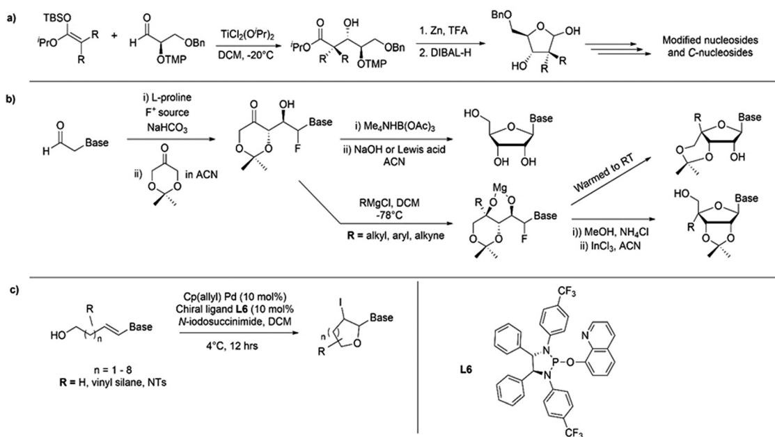
Fig. 2 Selected asymmetric syntheses of nucleosides and their analogues. (a) MacMillan's Mukaiyama aldol addition followed by ring closure and reduction. 36 (b) Britton's electrophilic \alpha -fluorination and aldol condensation followed by annulative fluoride displacement. 37 (c) Trost's palladium catalyzed formation of oxygen and nitrogen containing heterocycles bearing pyrimidine nucleobases. 38
