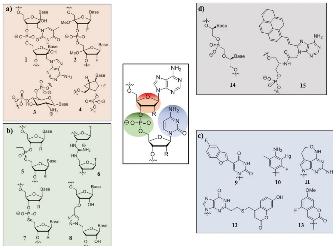
Fig. 1 Selected recent examples of chemical modifications introduced in nucleic acids. (a) sugar-modified nucleic acids including double-headed nucleotides ( 1 ), 20 2'-OMe,4'-F-modified ribonucleotides ( 2 ), 21 4',6'-glucosamino nucleic acids (GANA) ( 3 ), 22 and 2'-F-methanocarbazyclic nucleotides ( 4 ), 23 (b) backbone-modified nucleic acids including ( S )- P -ethyl-phosphonate nucleic acids ( 5 ), 24 deoxynucleic guanidine DNG ( 6 ), 25 phosphoroselenolate nucleic acid analogues ( 7 ), 26 and triazole-modified RNA ( 8 ); 27 (c) nucleobase modifications including 5-fluorobenzofuran-2'-deoxyuridine ( 9 ), 28 3-fluoro-6-methylanilinenucleotide ( 10 ) involved in Hg(II)-mediated base pairing, 29 bisversal pyrimidine analogue ( 11 ), 30 2-vinylhypoxanthine ( 12 ) further modified by the thiol-ene reaction, 31 and the fluorescent mimic of deoxycytidine containing a 5-fluoro-7-methoxy-coumarin moiety ( 13 ); 32 (d) nucleic acid analogues bearing modifications at multiple sites such as ( S )-ZNA ( 14 ) that contains an acyclic methylphosphonate backbone 33 and serinol nucleic acid (SNA) bearing a pyrene-modified adenine nucleobase ( 15 ). 34
