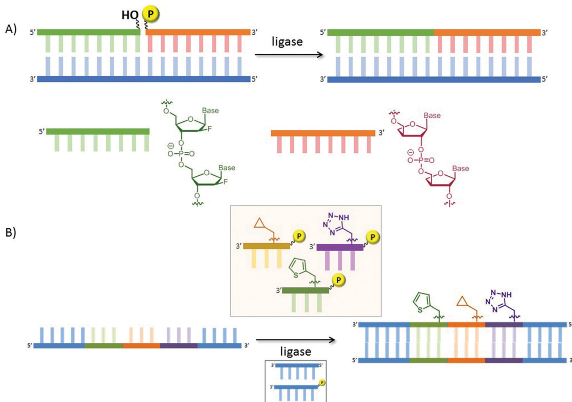
Fig. 11 Ligase-mediated synthesis of modified oligonucleotides: (A) two modified oligonucleotides (e.g. containing FANA or TNA units) can be ligated using a bridging DNA or XNA template; (B) multiple nucleotide codons containing base-modified nucleotides can be ligated to generate modified oligonucleotides.
