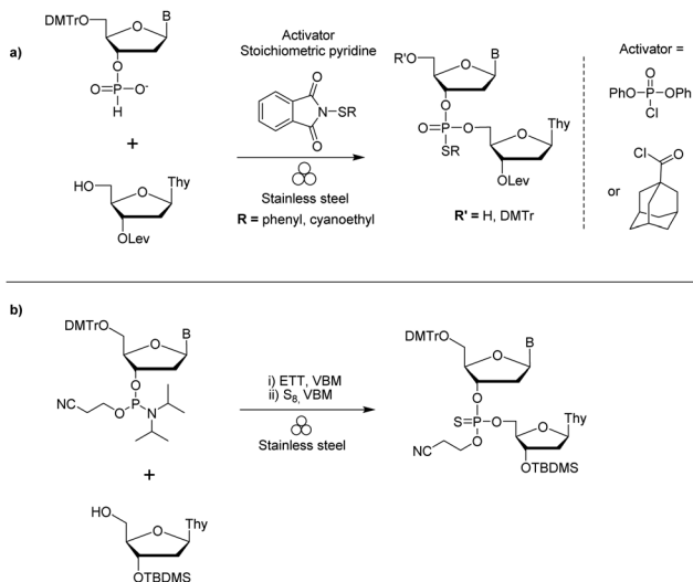
Fig. 9 Mechanochemical synthesis of short DNA fragments by vibration ball milling. (a) H-phosphonate approach using different activators and a sulfur transfer reagent. (b) Phosphoramidite approach using elemental sulfur for preparation of phosphorothioates. 213
