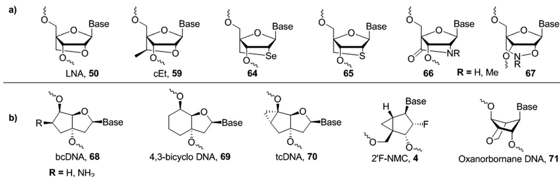
Fig. 21 Selected conformationally constrained nucleoside analogues. (a) LNA analogues (b) other bi- and tricyclic nucleoside analogues.
