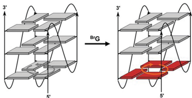
Fig. 14 G-tetrad polarity inversion in the parallel MYC quadruplex after substituting anti guanosine (gray) in the 5'-tetrad with syn 8-bromoguanosine (red), reproduced from ref. 306. 293 with permission from John Wiley and Sons.
