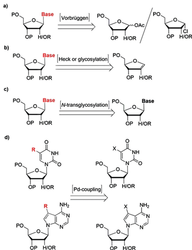
Fig. 3 Main synthetic pathways to nucleobase-modified purine and pyrimidine nucleoside analogues: (a) the Vorbrüggen nucleosidation reaction involving Lewis acid activated nucleophilic attack; 84 (b) the Pd-catalysed Heck reaction; 85,86 (c) chemoenzymatic transglycosylation methods; (d) Pd-assisted cross-coupling reactions with purine and pyrimidine precursors. 87
