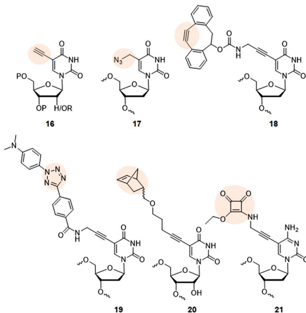
Fig. 5 Common nucleoside analogues used for biorthogonal labelling reactions including ethynyl-(deoxy)uridine (EdU/EU) 16 , 5-(Azidomethyl)-2'-deoxyuridine (AmdU) 17 , 94 dibenzocyclooctyne-modified deoxyuridine 5-DIBO-K 18 , 95 diaryltetrazole containing building block 19 , 96 norbornene-modified analogue 20 , 97 and nucleoside dC ESQ 21 equipped with a squaramate moiety. 98
