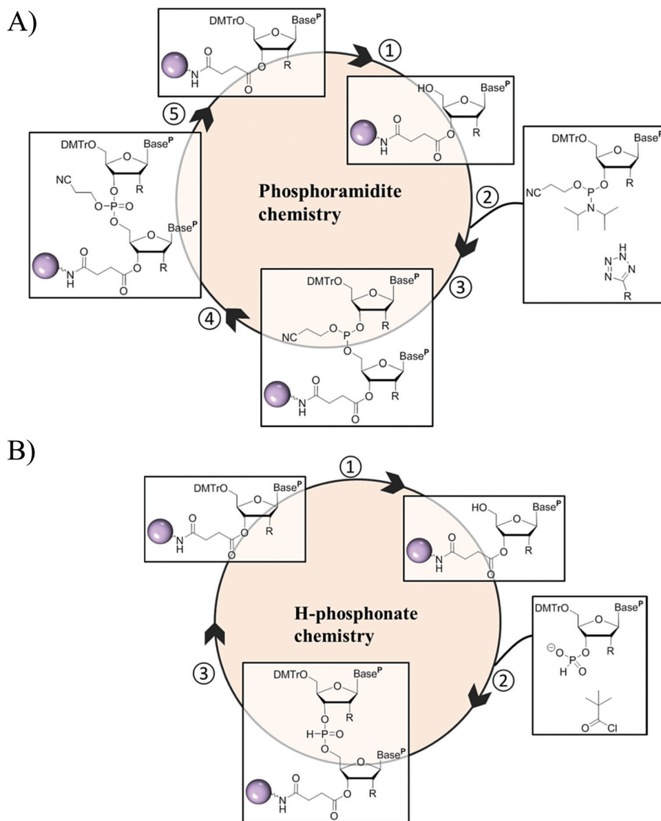
Fig. 7 Schematic representation of the main solid-support driven syntheses of oligonucleotides. (A) the synthetic cycle with phosphoramidite chemistry includes (1) deprotection of the DMTr groups; (2) condensation of the incoming phosphoramidite building block with a tetrazole activation step; (3) capping of the unreacted hydroxyl groups; (4) oxidation to P(v); and (5) either the cycle is repeated or the sequence is subjected to a global deprotection protocol. (B) The synthetic cycle with H-phosphonate chemistry includes (1) deprotection of the DMTr groups; (2) condensation of the incoming H-phosphonate building block in the presence of an activating agent such as pivaloyl chloride; (3) either the cycle is repeated or the sequence is subjected to an oxidation to P(v) followed by a global deprotection protocol.
