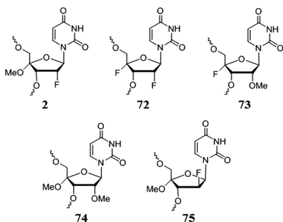
Fig. 22 Examples of 2',4'-modified nucleosides explored for potent siRNA activity. (2) 2'-deoxy-2'-fluoro-4'-methoxyribouridine; (71) 2'-deoxy-2',4'-difluorouridine; (72) 2'-methoxy-4'-fluorouridine; (73) 2',4'-dimethoxyribouridine; (74) 2'-deoxy-2'-fluoro-4'-methoxyarabinouridine.
