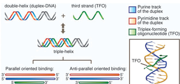
Fig. 18 Orientation of component strands of parallel and antiparallel triplexes. The inset cartoon is a triple helix structure derived from a NMR-structure (PDB-ID: 1BWG). Reproduced from ref. 325 with permission from Taylor & Francis.
