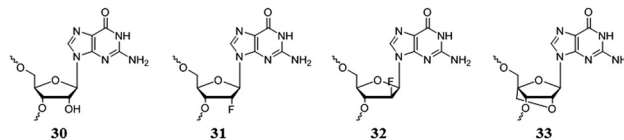
Fig. 15 Common anti guanosine analogues employed to stabilize parallel G-quadruplex topologies; riboguanosine (30); 307 2'-deoxy-2'-fluororiboguanosine (31); 297 2'-deoxy-2'-fluoroarabinoguanosine (32); 296–298,308 LNA guanosine (33). 299–301
