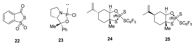
Fig. 8 Structures of the Beaucage reagent ( 22 ) and of chiral precursors ( 23–25 ) used in the stereocontrolled synthesis of PS-oligonucleotides.
