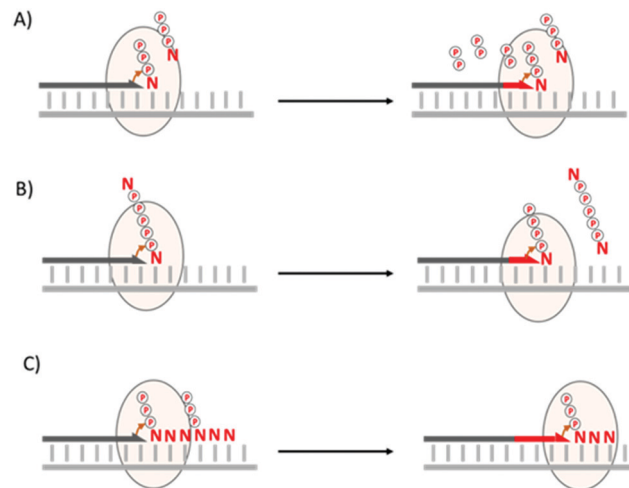
Fig. 10 Schematic representation of primer extension reaction with (A) DNA polymerases using natural dN*TPs and formation of pyrophosphate as by-product; (B) DNA polymerases and pentaphosphate deoxynucleotide dimers which produces a nucleotide tetraphosphate as by-product (shown next to the primer elongated by one nucleotide on the right hand side), itself a substrate for polymerases and incorporated into DNA. A second, incoming pentaphosphate deoxynucleotide dimer then allows DNA synthesis to continue; (C) a ribozyme and nucleotide triplet building blocks.
