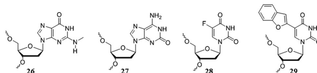
Fig. 13 Selected modified nucleosides that stabilized the G-quadruplexes they were studied in; (26) N 2 -methylguanosine; 284,287 (27) isoguanosine; 288 (28) 5-fluorouridine; 285 (29) 5-(benzofuran-2-yl)uracil (5bu). 286
