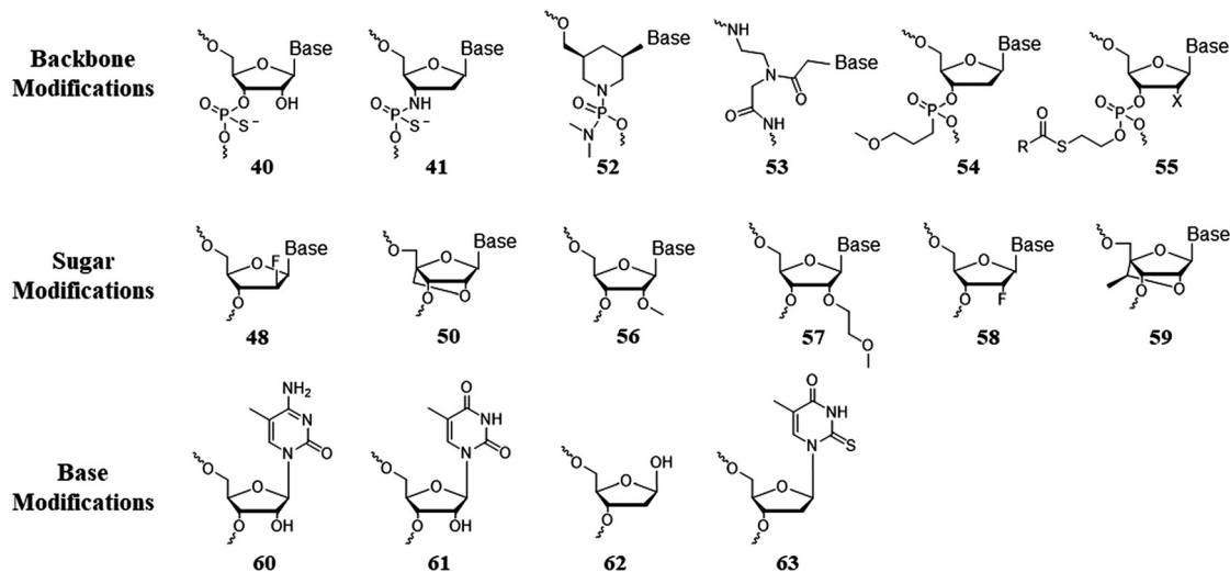
Fig. 20 Selected examples of prominent nucleoside modifications used in ASO and siRNA; (40) Phosphorothioate (PS) linkage; (41) N3'-P5' thiophosphoroamidate linkage; (52) morpholino phosphorodiamidate (PMO) backbone; (53) peptide nucleic acid (PNA) backbone; (54) methoxypropylphosphonate (MOP) linkage; (55) phosphotriester linkages; (48) 2'-deoxy-2'-fluoroarabino (2'-F-ara); (50) locked nucleic acid (LNA) (56) 2'-O-methyl (2'-OMe); (57) 2'-O-methoxyethyl (2'-MOE); (58) 2'-deoxy-2'-fluoro (2'-F); (59) S-constrained ethyl bridged nucleic acid (cEt); (60) 5-methylcytosine; (61) 5-methyluracil (thymine); (62) abasic nucleoside; (63) 2-thiothymine.
