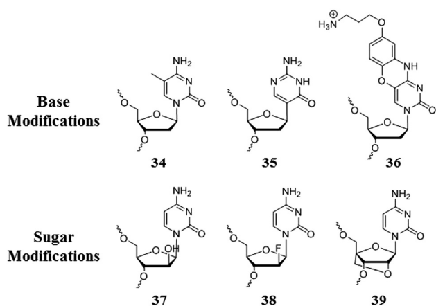
Fig. 17 Selected modified nucleosides that resulted in i-motif stabilization; (34) 5-methylcytidine; 313 (35) pseudoisocytidine; 314 (36) iClamp; 315 (37) 2'-arabinocytidine; 316 (38) 2'-deoxy-2'-fluoroarabinocytidine; 302,317 (39) LNA-cytidine. 318
