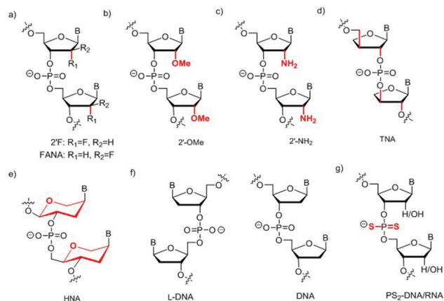
Fig. 24 Chemical structure of sugar and backbone modifications used in aptamer selections; (a) 2'-fluoro-modification; (b) 2'-methoxy-modification; (c) 2'-amino-modification; (d) threose nucleic acid (TNA); (e) 1,5-anhydrohexitol nucleic acids (HNA); (f) Spiegelmers (L-DNA); (g) phosphorodithioates (PS 2 ).
