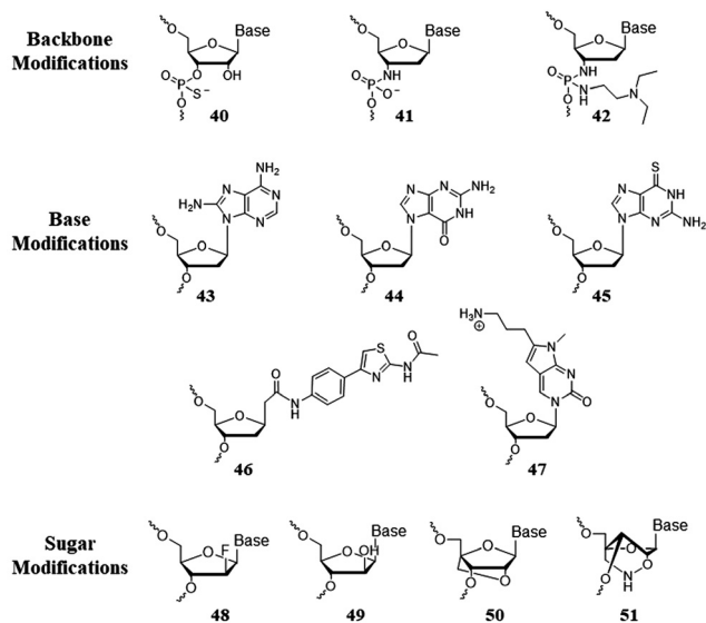
Fig. 19 Selected nucleoside modifications that resulted in triplex stabilization; (40) Phosphorothioate linkage; 326 (41) N3' → P5' phosphoramidate linkage; 327 (42) DEED phosphoramidate linkage; 328 (43) 8-aminoadenine; 329 (44) N 7 -glycosylated guanine; 330 (45) 6-thioguanine; 331 (46) S; 332 (47) A PP ; 333,334 (48) 2'-deoxy-2'-fluoroarabinose modification; 335 (49) 2'-arabinose modification; 336 (50) LNA; 337 (51) 2',4'-BNA NC [NH]. 338
