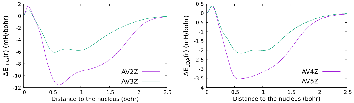
FIG. 8. Behavior of \Delta E_{\text{LDA}}^{\text{B}}(r) for the AV2Z and AV3Z basis sets (left plot) and AV4Z and AV5Z basis sets (right plot) for the oxygen atom.
