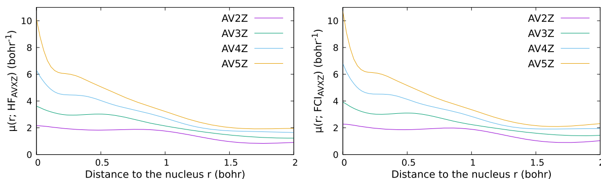
FIG. 3. Local range-separated parameter \mu(\mathbf{r}; \Psi^{\mathcal{B}}) for the helium atom for different aug-cc-pVXZ basis sets ( X = 2, 3, 4, 5 ) as a function of the position \mathbf{r} along the diagonal of the xy plane. The curve on the left is when using the HF wave function for \Psi^{\mathcal{B}} , and the curve on the right is when using the FCI wave function for \Psi^{\mathcal{B}} .
