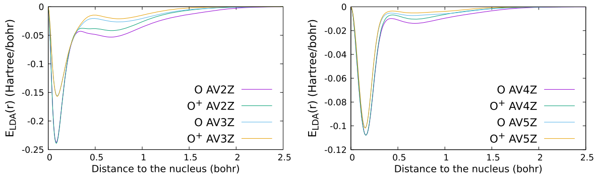
FIG. 7. Behavior of \bar{E}_{\text{LDA}}^{\text{B}}(r) for the AV2Z and AV3Z basis sets (left plot) and AV4Z and AV5Z basis sets (right plot) for the oxygen atom and its first cation.
