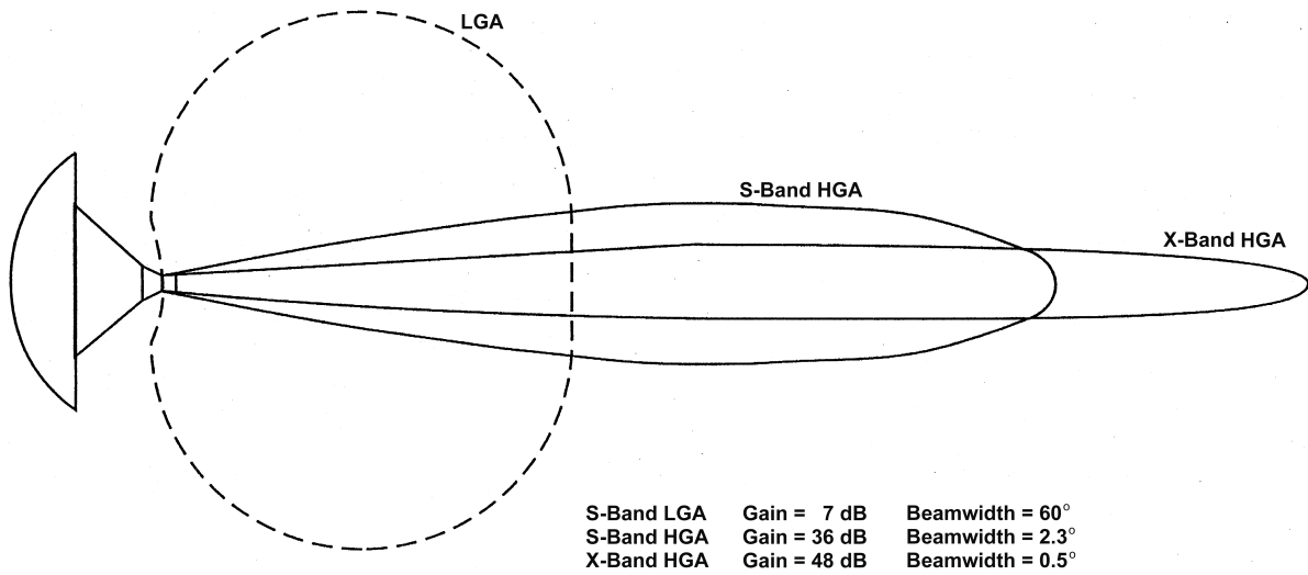
Fig. 3-2. Voyager SXA patterns and beamwidths.
